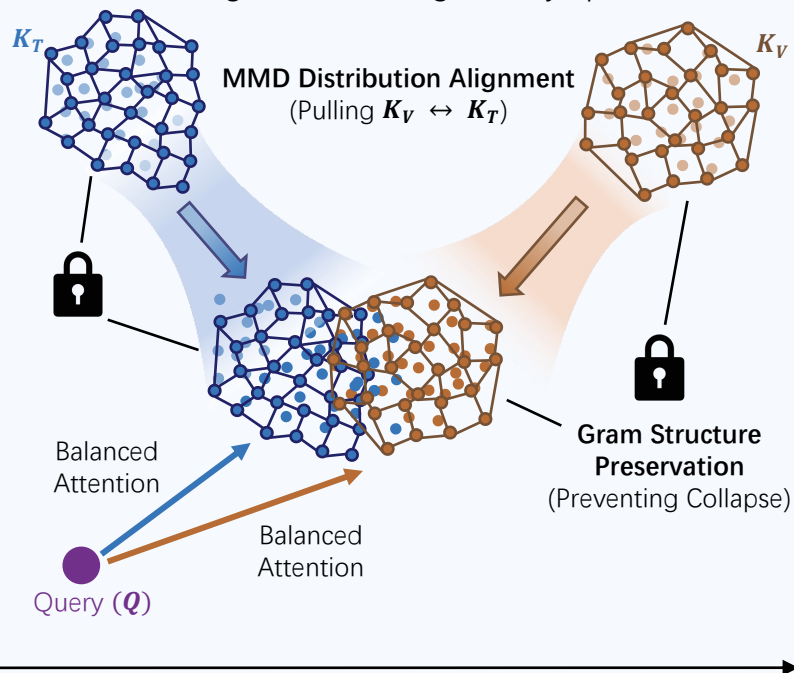
Training Process & Aligned Key Space
